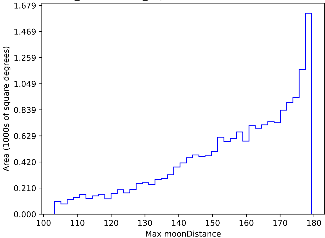
weather_cloudso2v3.4_10yrs WFD r band: Max moonDistance
