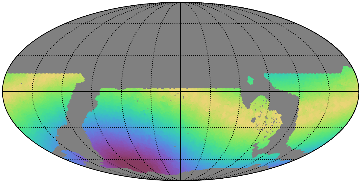
weather_cloudso2v3.4_10yrs WFD i band: Max moonDistance
