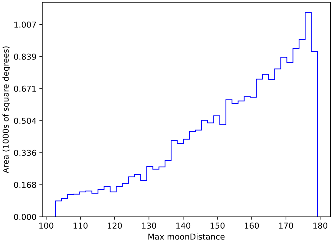
weather_cloudso2v3.4_10yrs WFD g band: Max moonDistance
