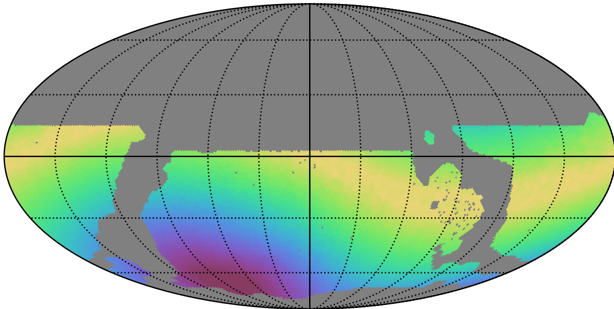
weather_cloudso2v3.4_10yrs WFD all bands: Max moonDistance
