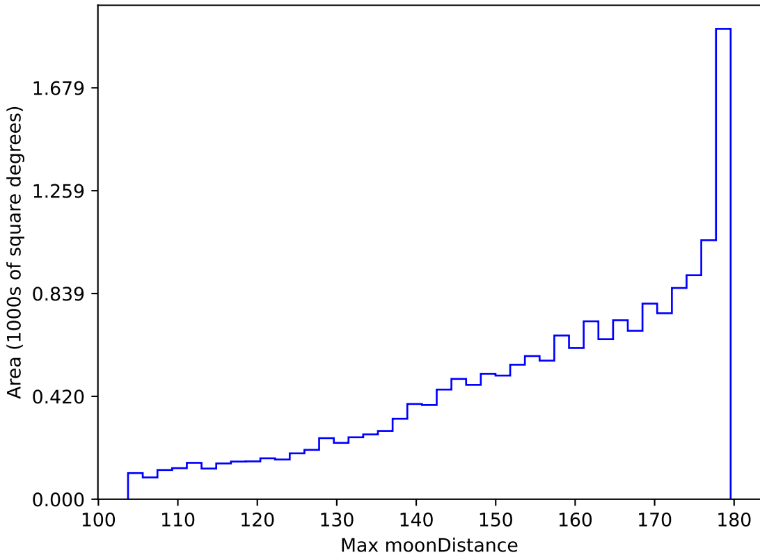
weather_cloudso2v3.4_10yrs WFD all bands: Max moonDistance
