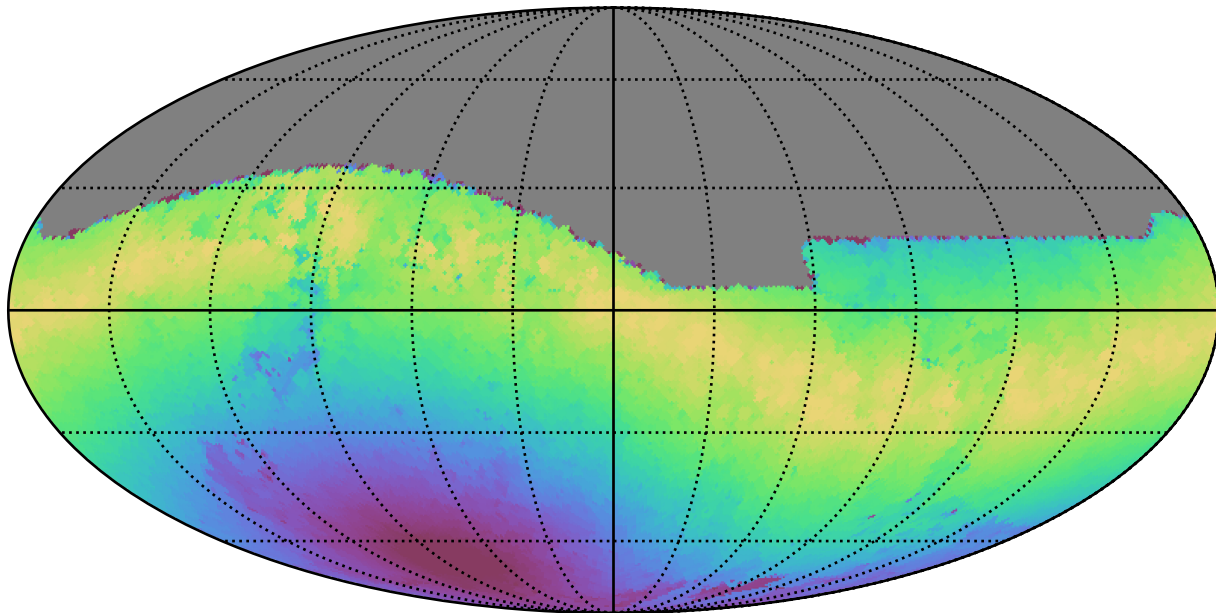
weather_cloudso2v3.4_10yrs All sky z band: Max moonDistance
