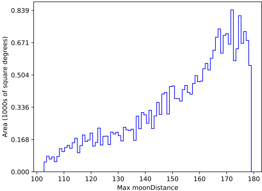
weather_cloudso2v3.4_10yrs All sky z band: Max moonDistance
