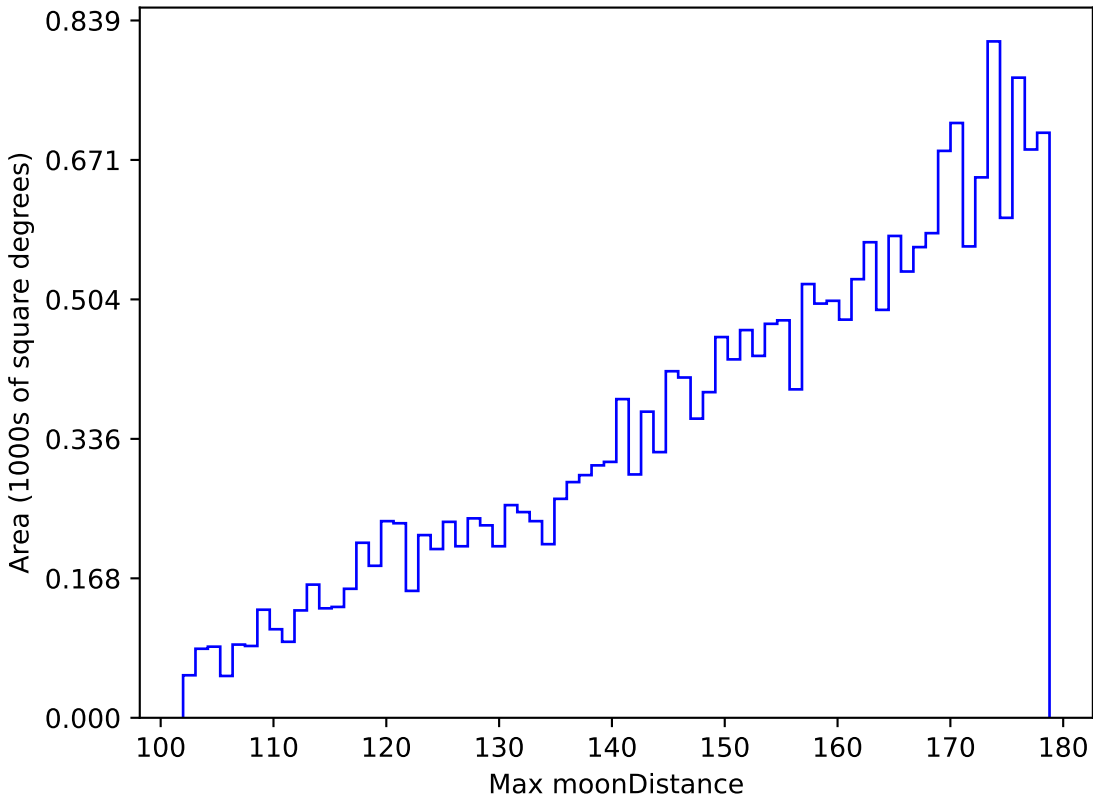
weather_cloudso2v3.4_10yrs All sky u band: Max moonDistance
