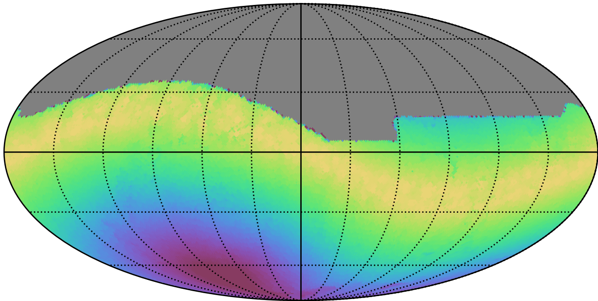
weather_cloudso2v3.4_10yrs All sky r band: Max moonDistance
