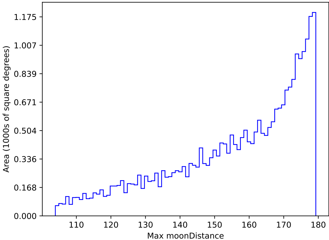
weather_cloudso2v3.4_10yrs All sky r band: Max moonDistance
