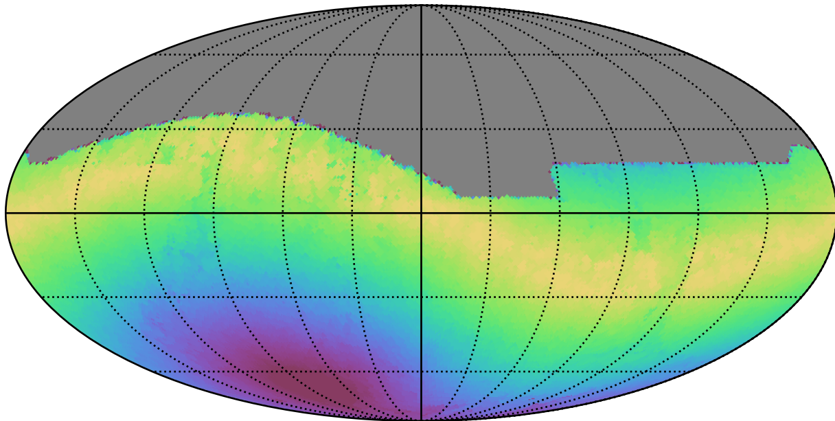
weather_cloudso2v3.4_10yrs All sky i band: Max moonDistance
