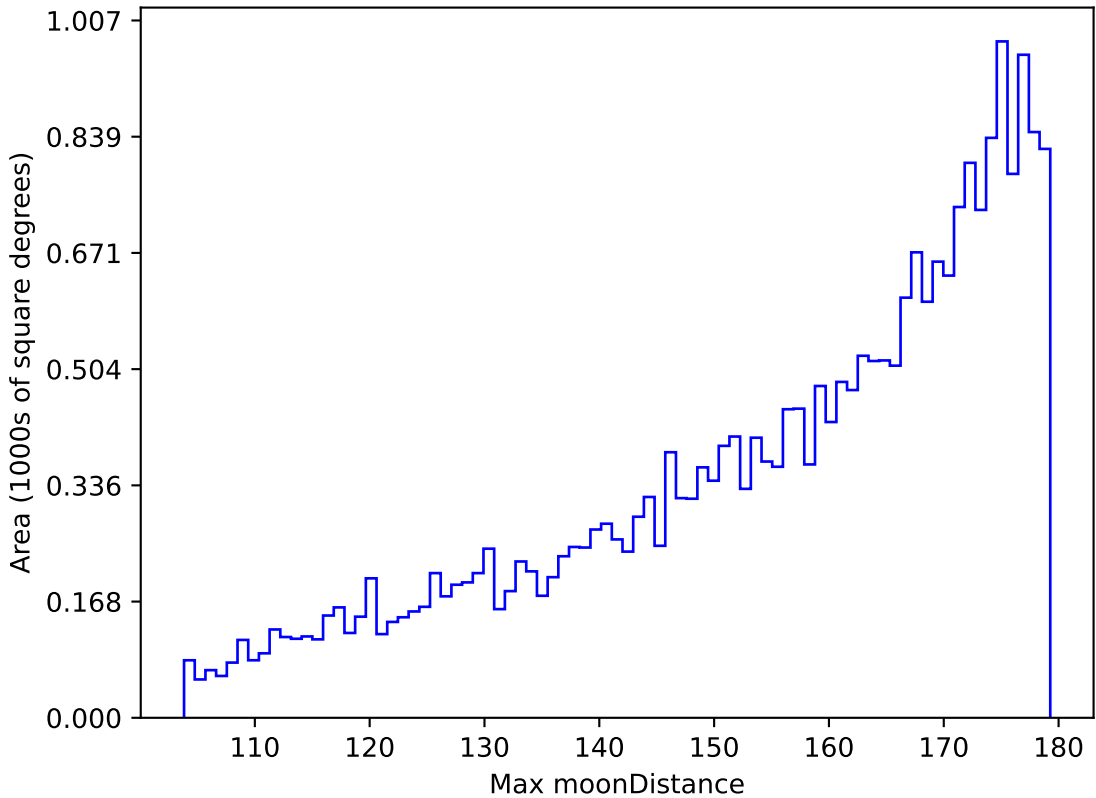
weather_cloudso2v3.4_10yrs All sky i band: Max moonDistance
