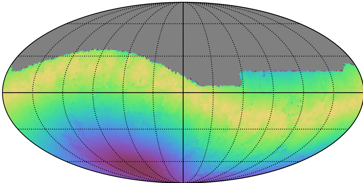
weather_cloudso2v3.4_10yrs All sky g band: Max moonDistance
