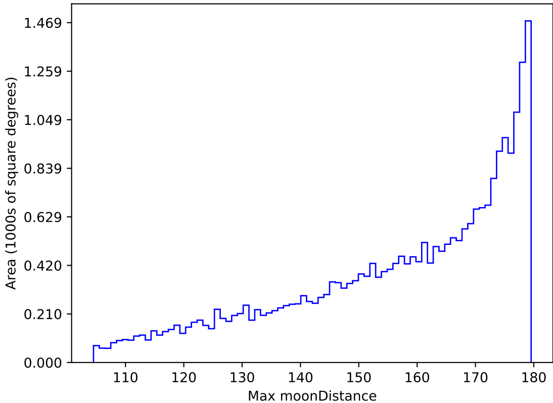
weather_cloudso2v3.4_10yrs All sky all bands: Max moonDistance
