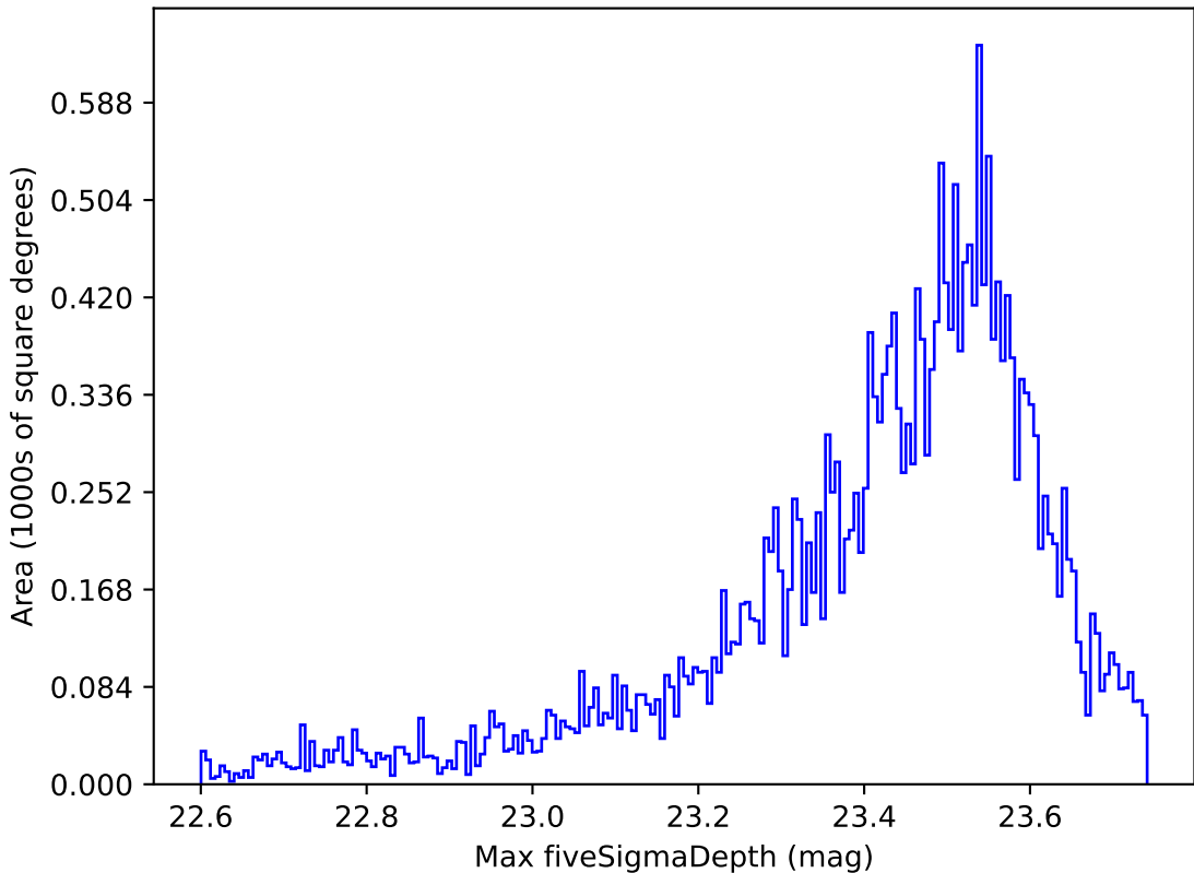
weather_cloudso2v3.4_10yrs Yr 1 z band: Max fiveSigmaDepth
