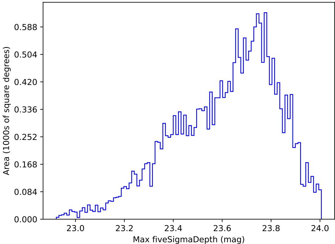
weather_cloudso2v3.4_10yrs Yr 1 u band: Max fiveSigmaDepth
