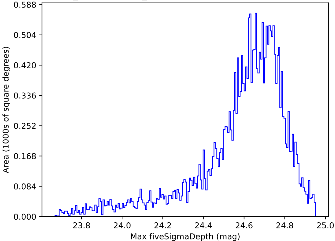
weather_cloudso2v3.4_10yrs Yr 1 r band: Max fiveSigmaDepth
