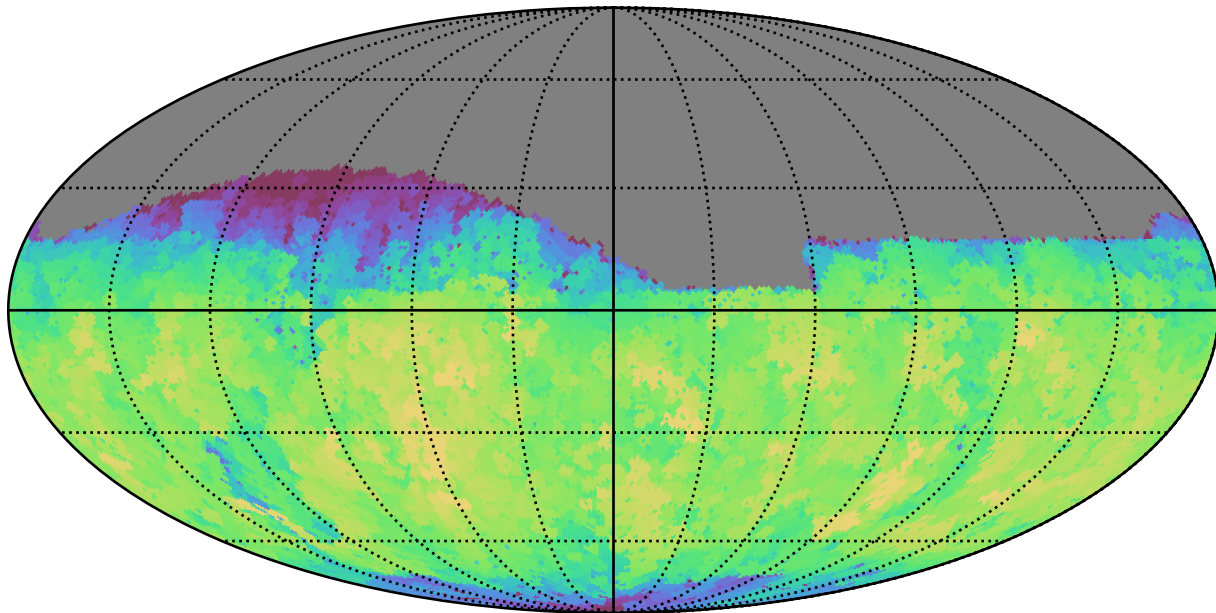
weather_cloudso2v3.4_10yrs Yr 1 i band: Max fiveSigmaDepth
