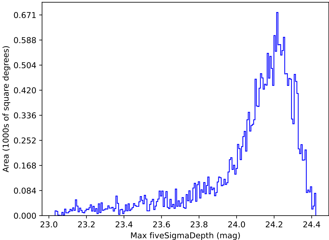
weather_cloudso2v3.4_10yrs Yr 1 i band: Max fiveSigmaDepth
