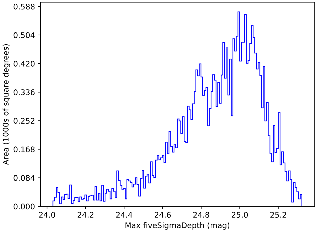
weather_cloudso2v3.4_10yrs Yr 1 g band: Max fiveSigmaDepth
