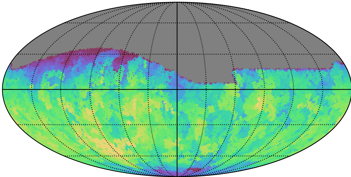
weather_cloudso2v3.4_10yrs Yr 1 all bands: Max fiveSigmaDepth
