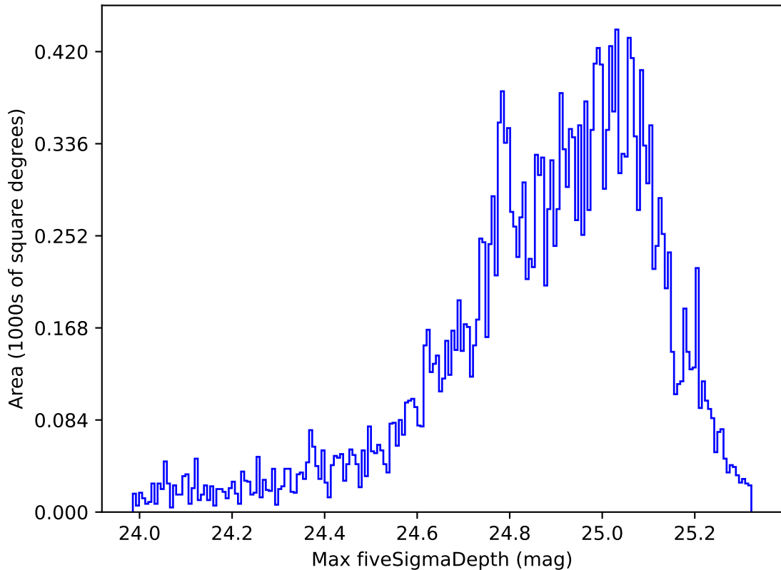
weather_cloudso2v3.4_10yrs Yr 1 all bands: Max fiveSigmaDepth
