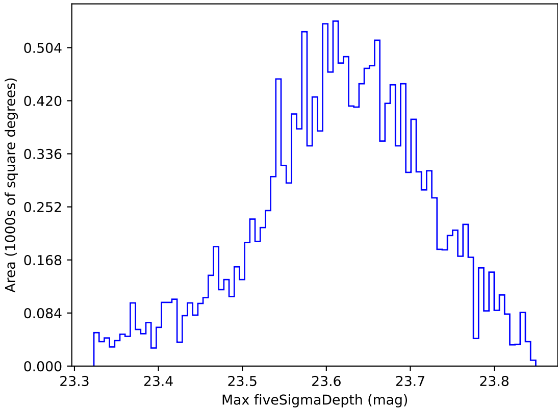
weather_cloudso2v3.4_10yrs WFD z band: Max fiveSigmaDepth
