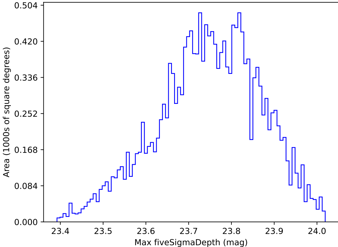
weather_cloudso2v3.4_10yrs WFD u band: Max fiveSigmaDepth
