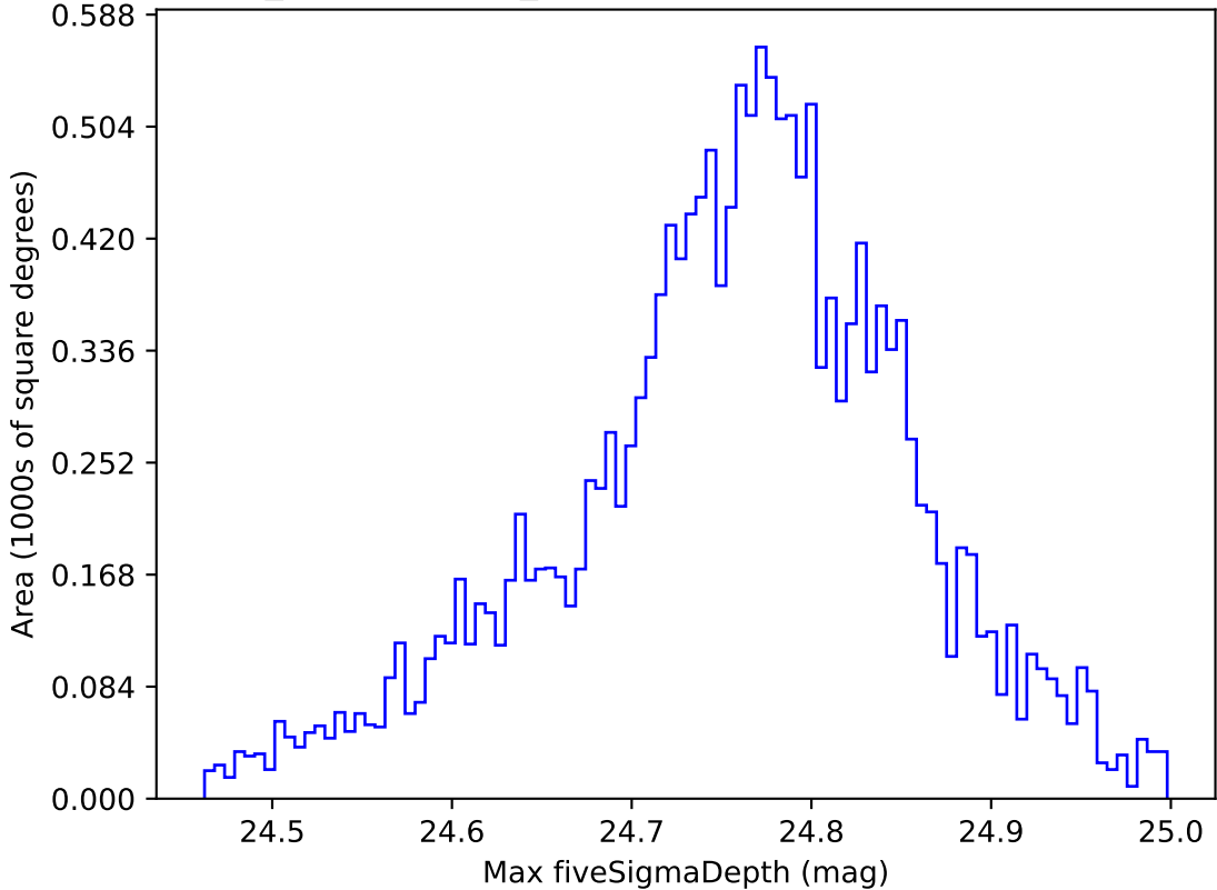
weather_cloudso2v3.4_10yrs WFD r band: Max fiveSigmaDepth
