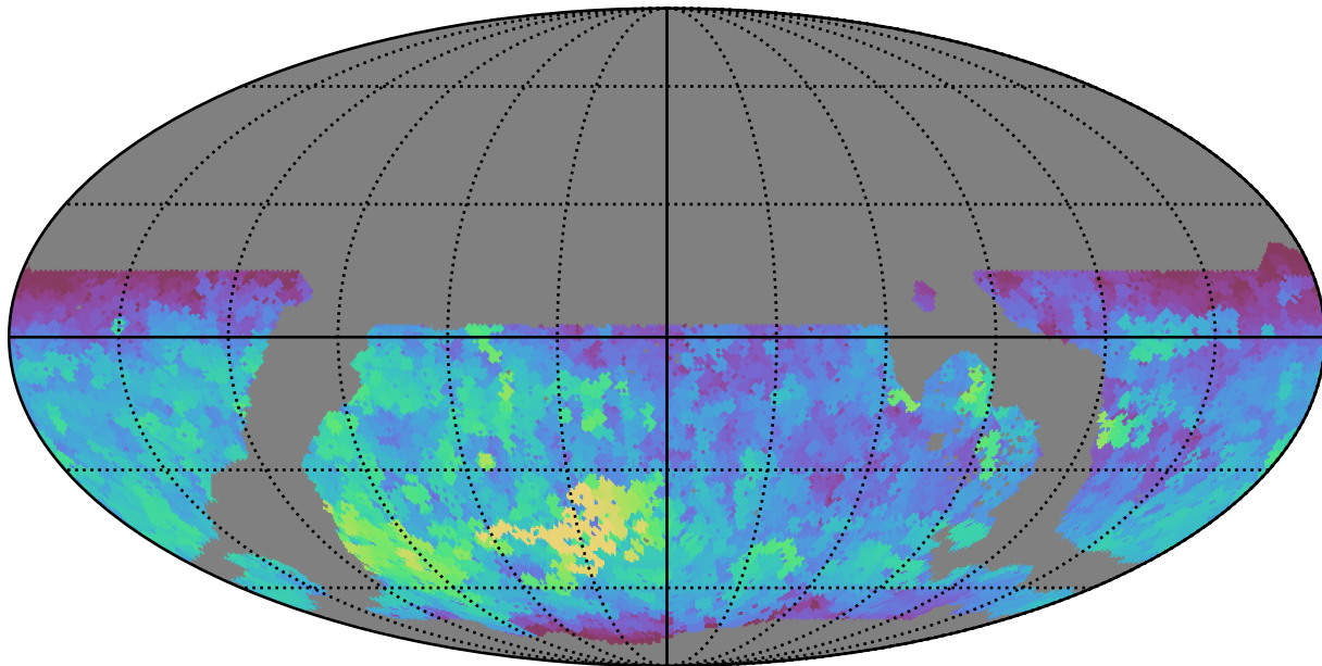
weather_cloudso2v3.4_10yrs WFD g band: Max fiveSigmaDepth
