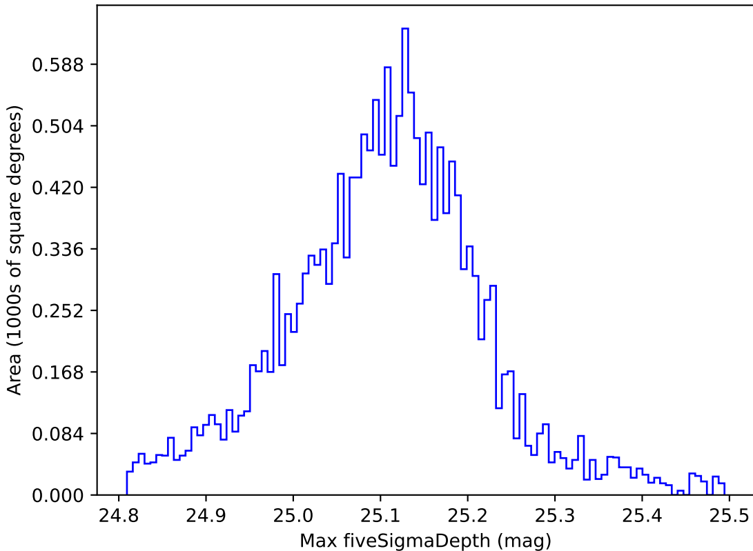
weather_cloudso2v3.4_10yrs WFD g band: Max fiveSigmaDepth
