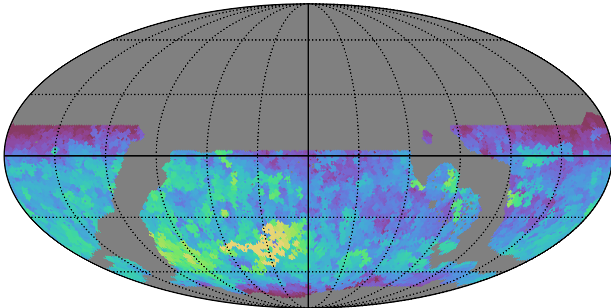
weather_cloudso2v3.4_10yrs WFD all bands: Max fiveSigmaDepth
