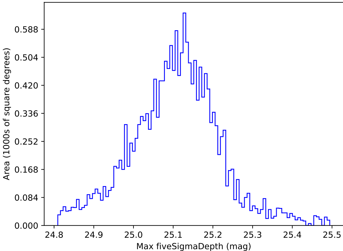
weather_cloudso2v3.4_10yrs WFD all bands: Max fiveSigmaDepth
