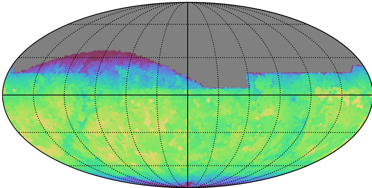
weather_cloudso2v3.4_10yrs All sky z band: Max fiveSigmaDepth
