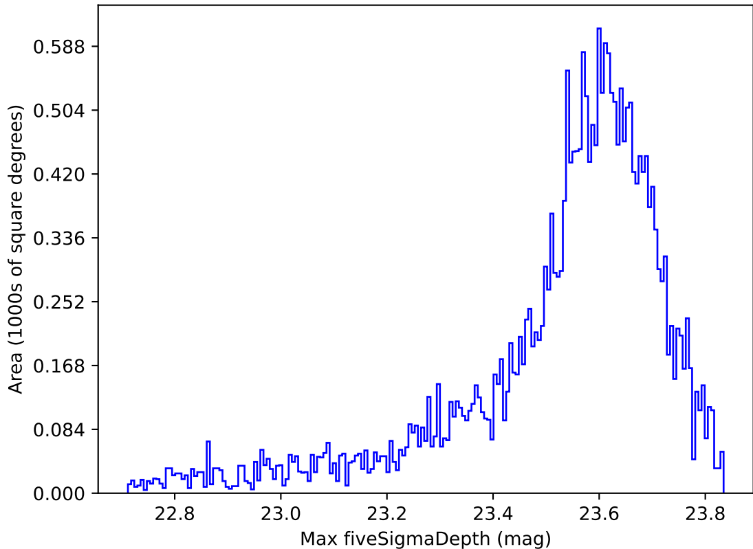
weather_cloudso2v3.4_10yrs All sky z band: Max fiveSigmaDepth
