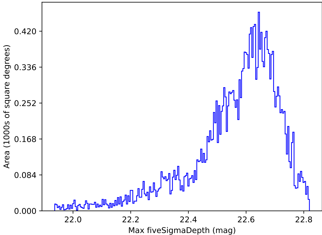
weather_cloudso2v3.4_10yrs All sky y band: Max fiveSigmaDepth
