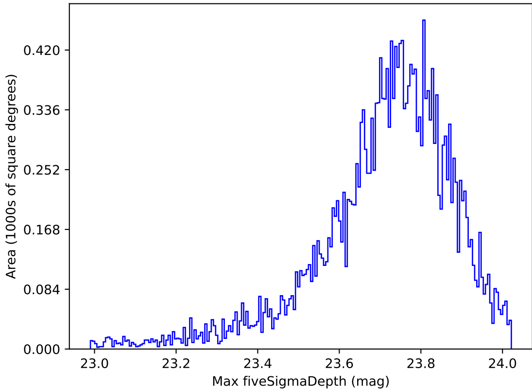
weather_cloudso2v3.4_10yrs All sky u band: Max fiveSigmaDepth
