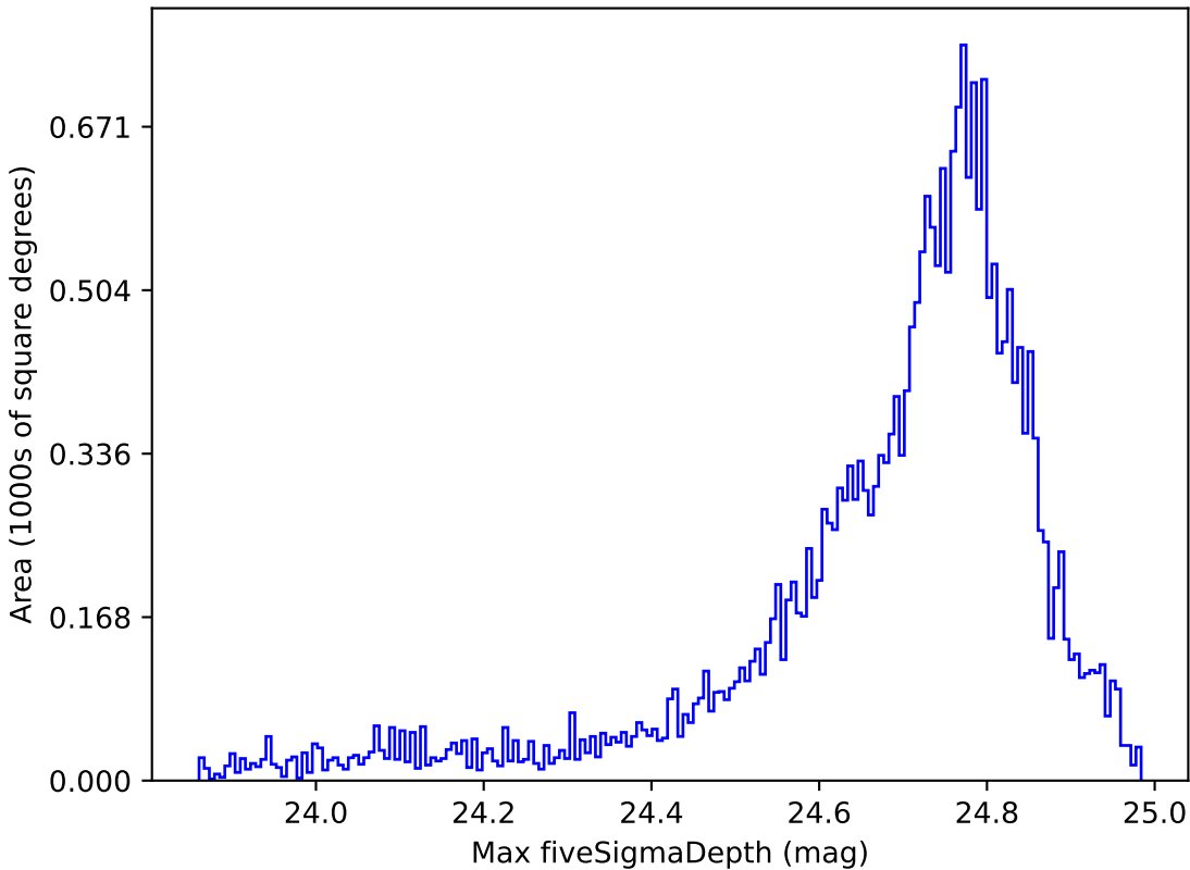
weather_cloudso2v3.4_10yrs All sky r band: Max fiveSigmaDepth
