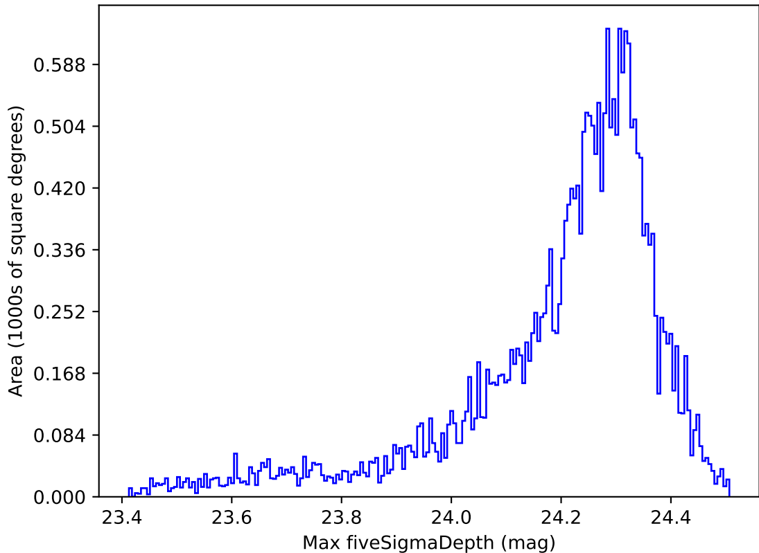
weather_cloudso2v3.4_10yrs All sky i band: Max fiveSigmaDepth
