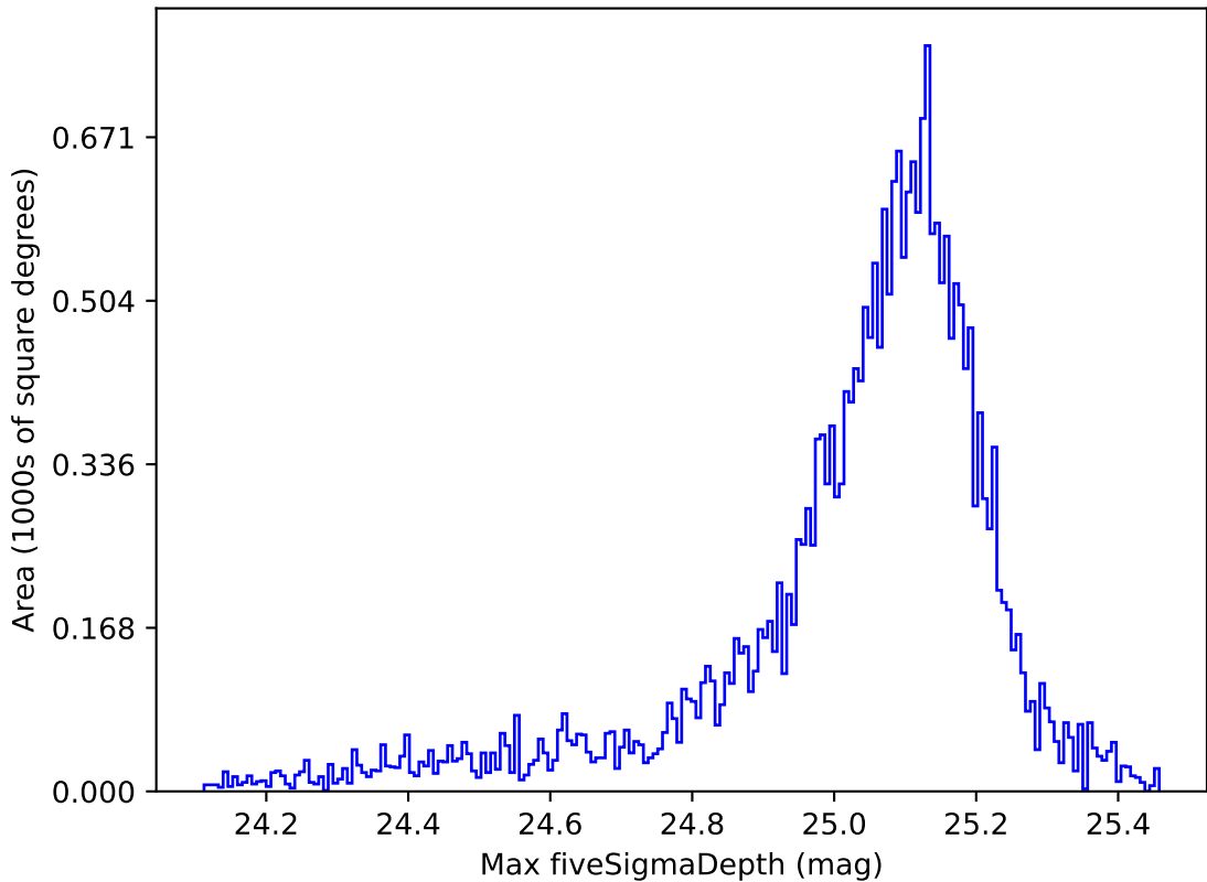
weather_cloudso2v3.4_10yrs All sky all bands: Max fiveSigmaDepth
