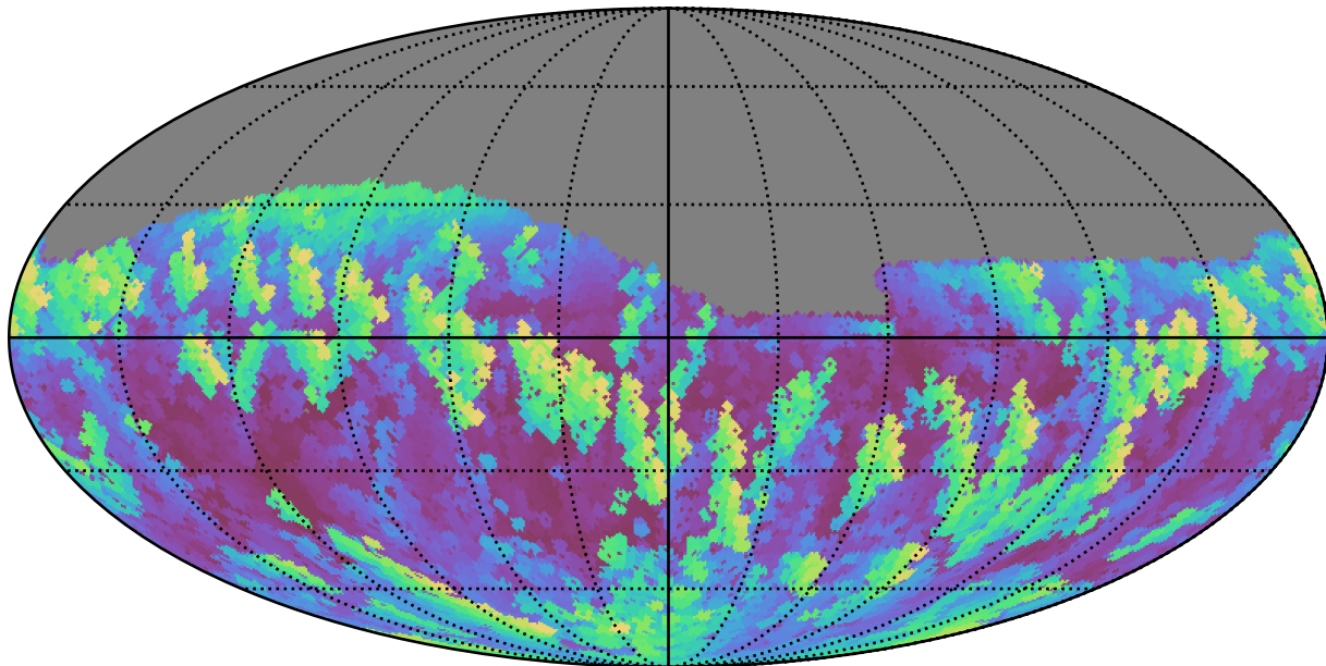
weather_cloudso2v3.4_10yrs Yr 1 z band: Max airmass
