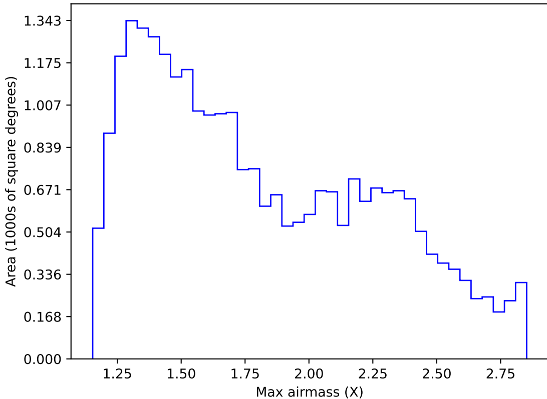
weather_cloudso2v3.4_10yrs Yr 1 z band: Max airmass
