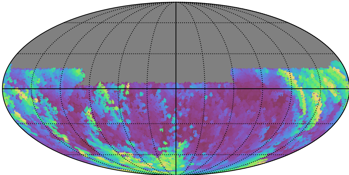
weather_cloudso2v3.4_10yrs Yr 1 y band: Max airmass
