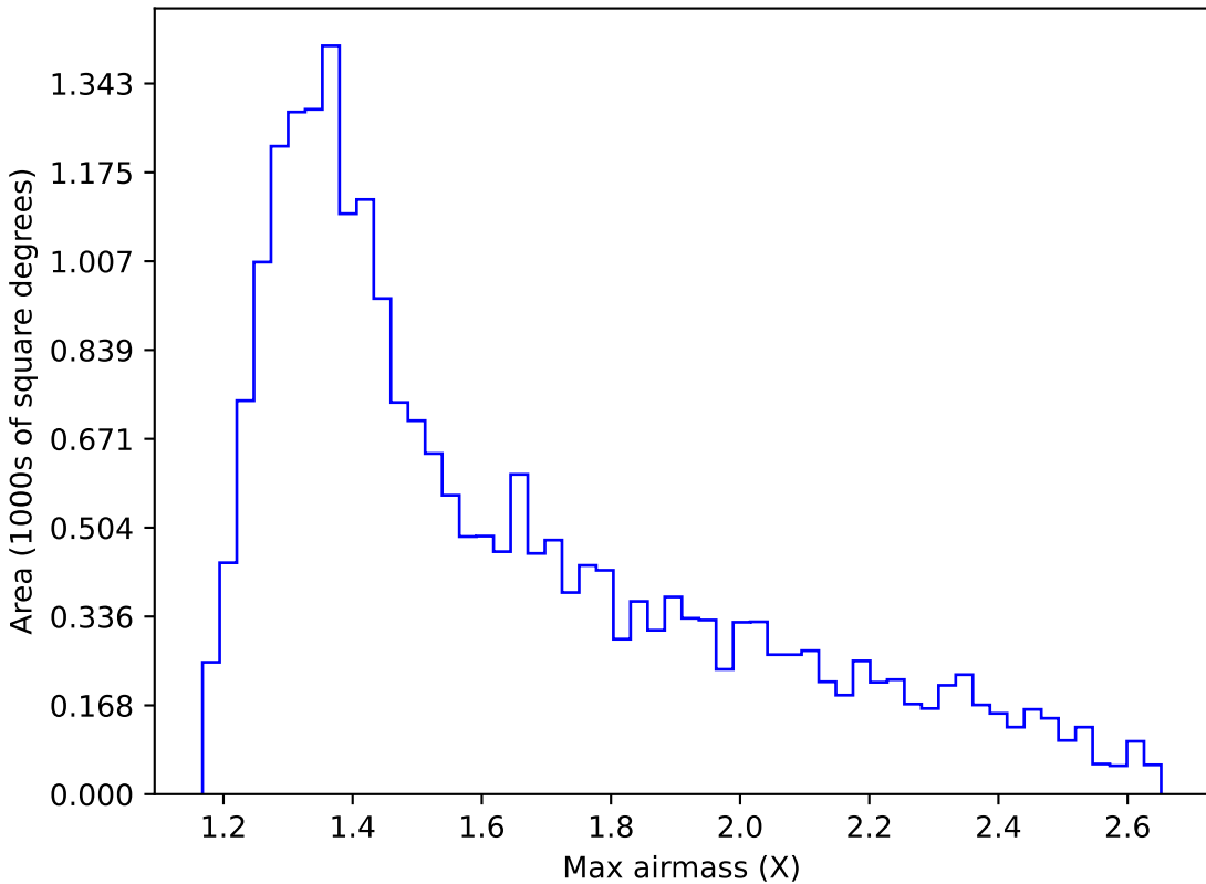
weather_cloudso2v3.4_10yrs Yr 1 y band: Max airmass
