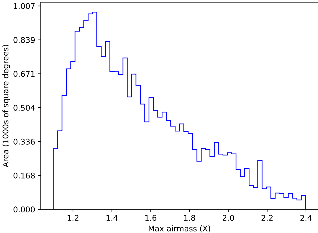
weather_cloudso2v3.4_10yrs Yr 1 u band: Max airmass
