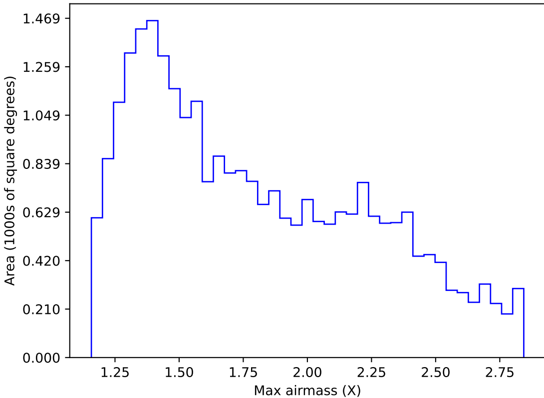
weather_cloudso2v3.4_10yrs Yr 1 i band: Max airmass
