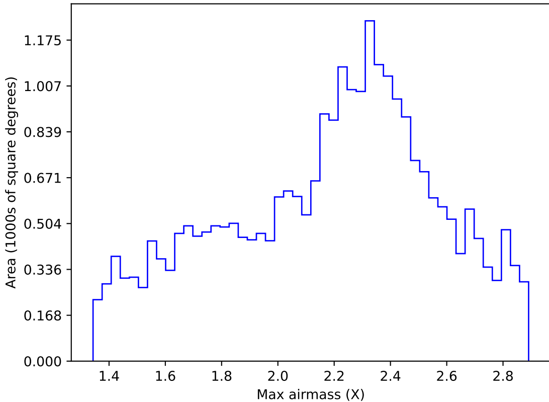
weather_cloudso2v3.4_10yrs Yr 1 all bands: Max airmass
