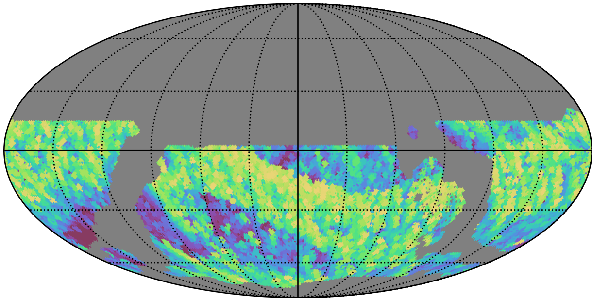
weather_cloudso2v3.4_10yrs WFD z band: Max airmass
