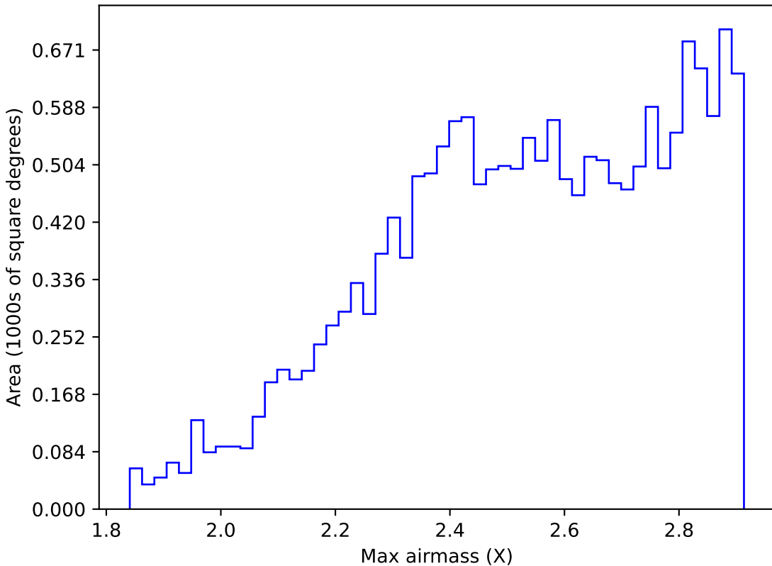
weather_cloudso2v3.4_10yrs WFD z band: Max airmass
