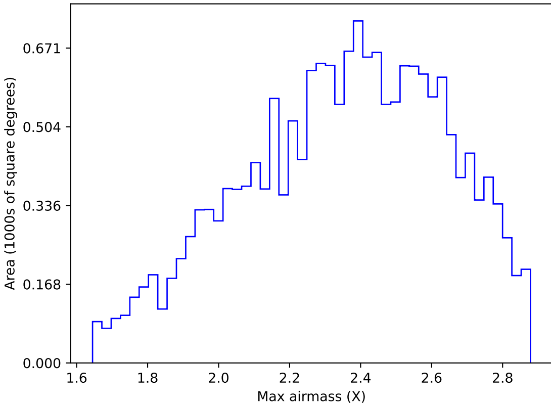
weather_cloudso2v3.4_10yrs WFD y band: Max airmass
