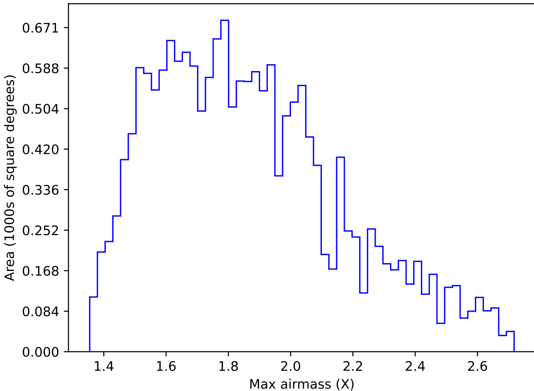
weather_cloudso2v3.4_10yrs WFD u band: Max airmass
