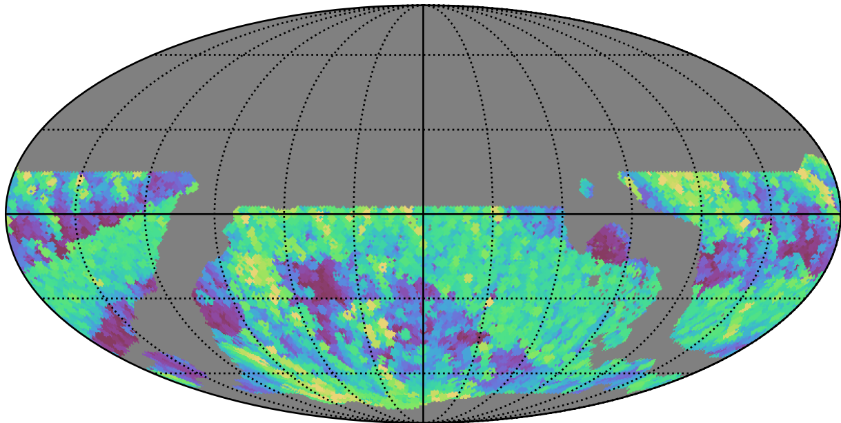
weather_cloudso2v3.4_10yrs WFD r band: Max airmass
