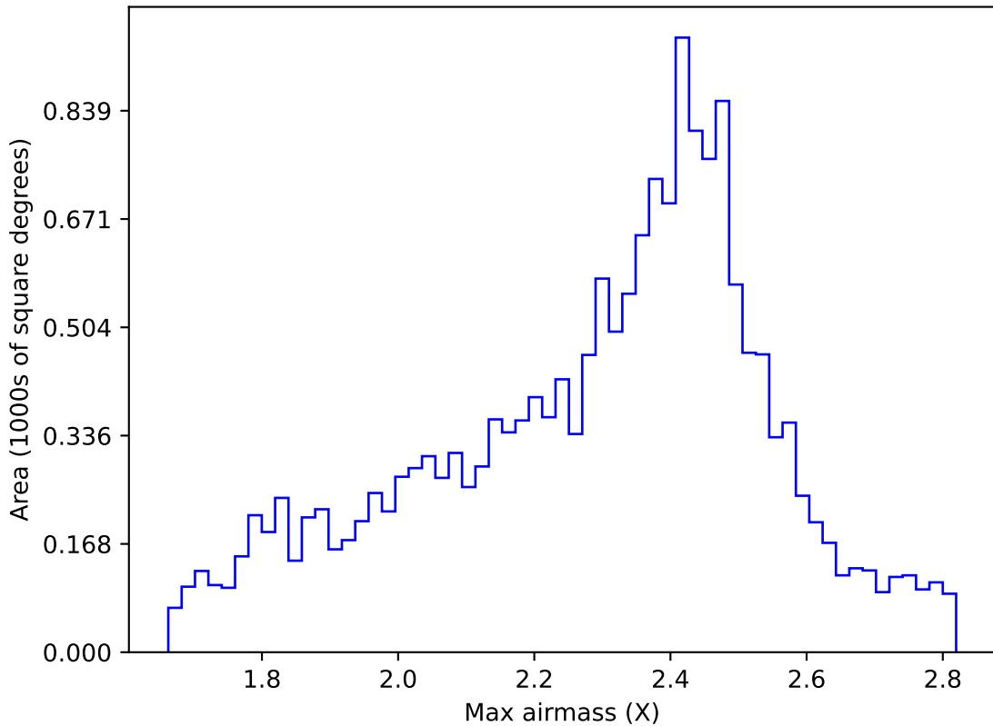
weather_cloudso2v3.4_10yrs WFD r band: Max airmass
