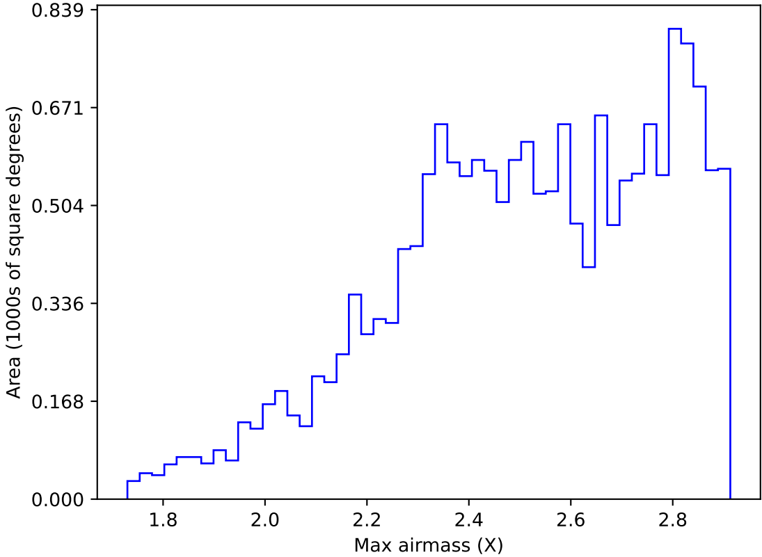
weather_cloudso2v3.4_10yrs WFD i band: Max airmass
